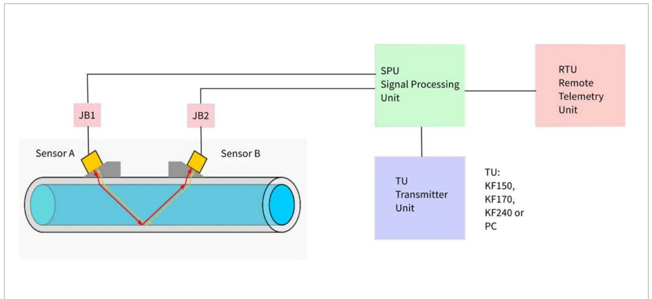
KATflow G system diagramm
